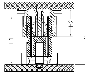
Assembly
